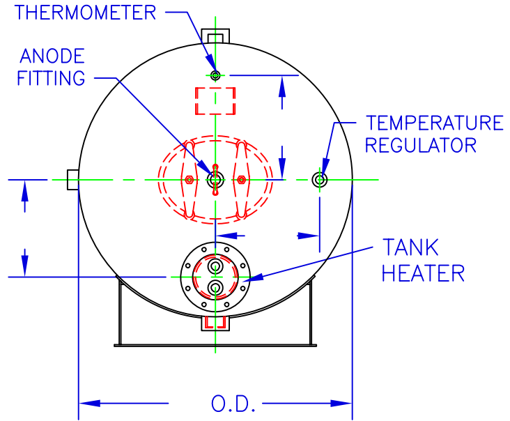
VIEW 'A-A'
